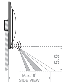
Wall Mount Sensor Detection Range
