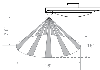
Ceiling Mount Sensor Detection Range
